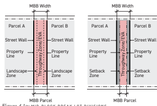
Figure 4.1a: MID-BLOCK BREAK LOT DIVISIONS
