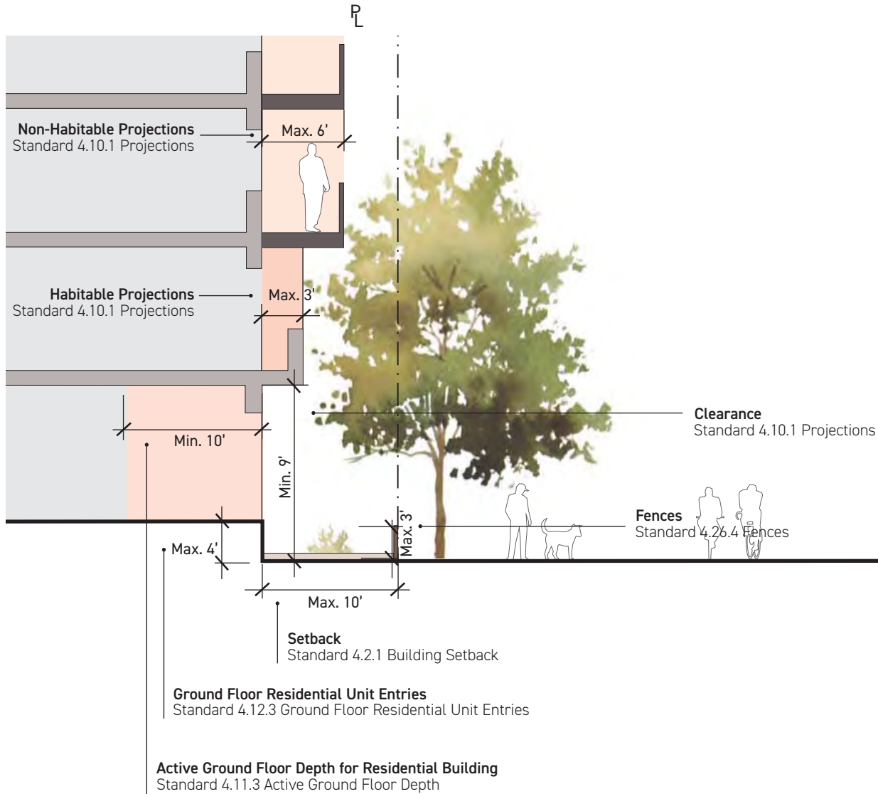
Figure 4.26e: SETBACK ZONE 4 (0' MIN./10' MAX.)
