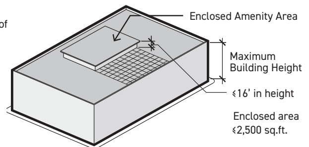
Figure 4.4h: BUILDING HEIGHT EXCEPTIONS ENCLOSED AMENITY AREA
