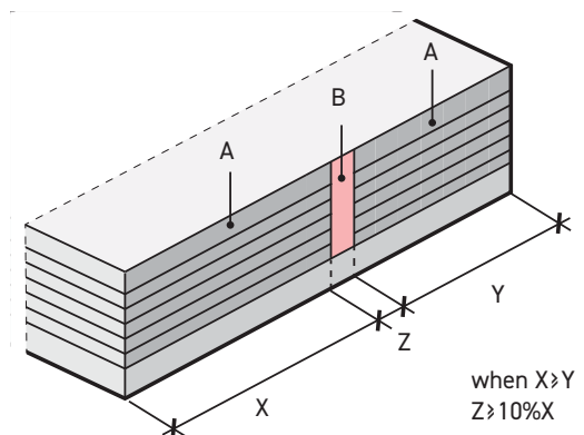
Figure 4.7i: EXAMPLE OF FV2 VERTICAL VARIATION B
