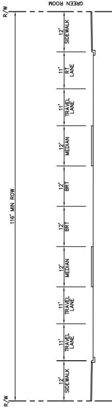
Crisp Road, west of Cochrane Street
