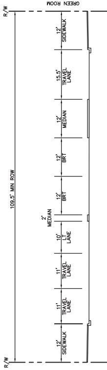
Crisp Road, east of H Street
