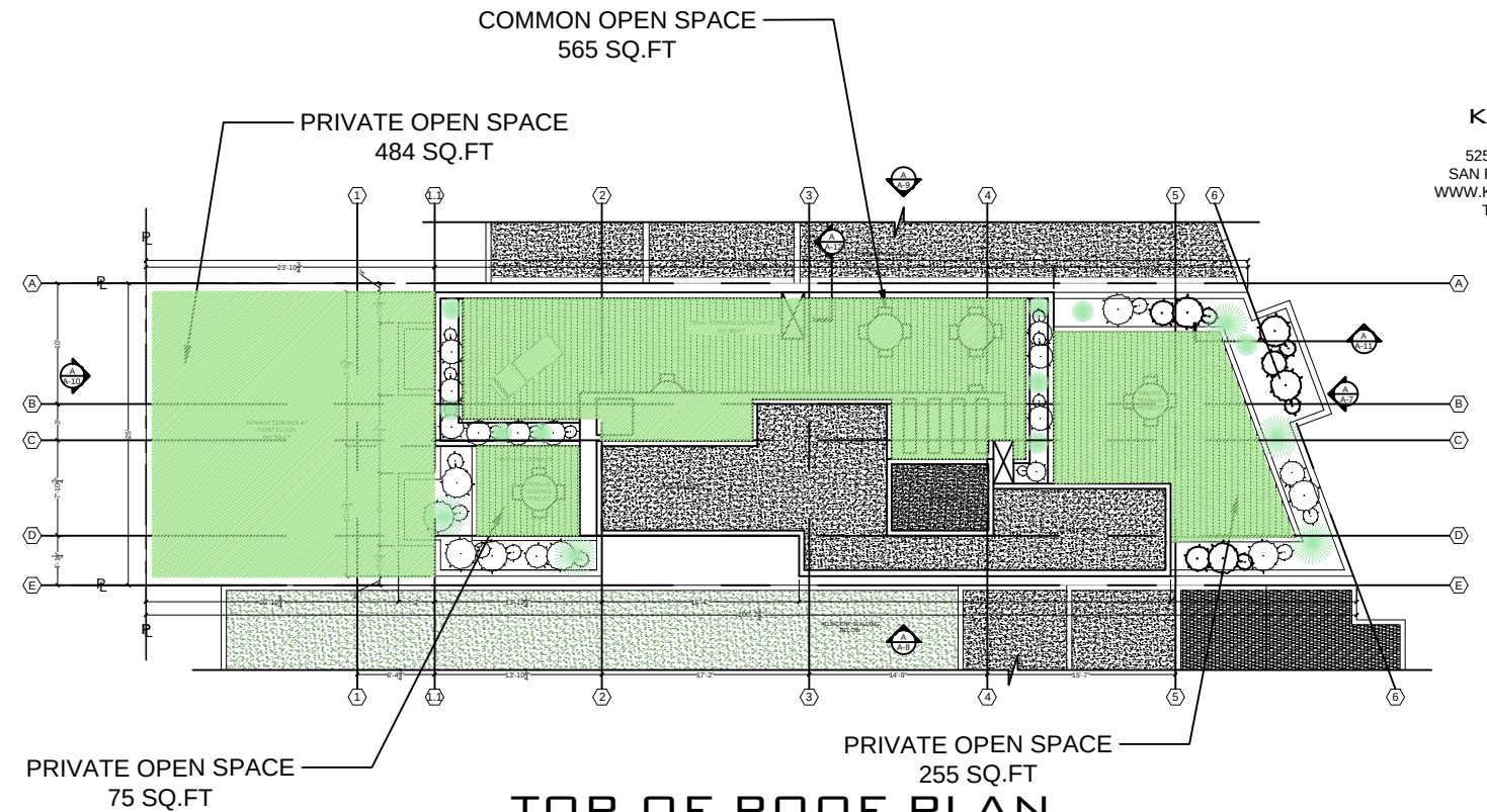
TOP OF ROOF PLAN ALL LEVELS PRIVATE & COMMON OPEN SPACES
